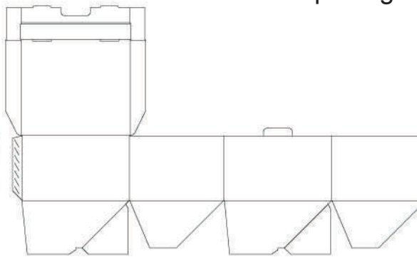
Box with snap-on lid with 3-point adhesion
