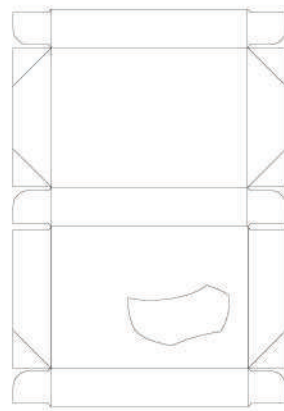
6 point glued box
