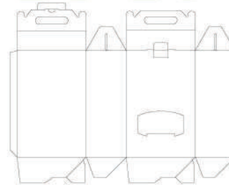
Bag type box with 3 point sealing
