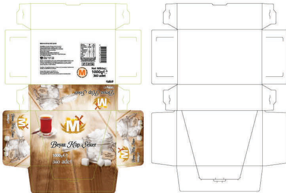
Locked sugar cube box
