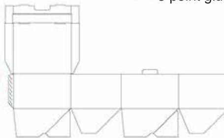
Box with snap-on lid with 3-point adhesion
